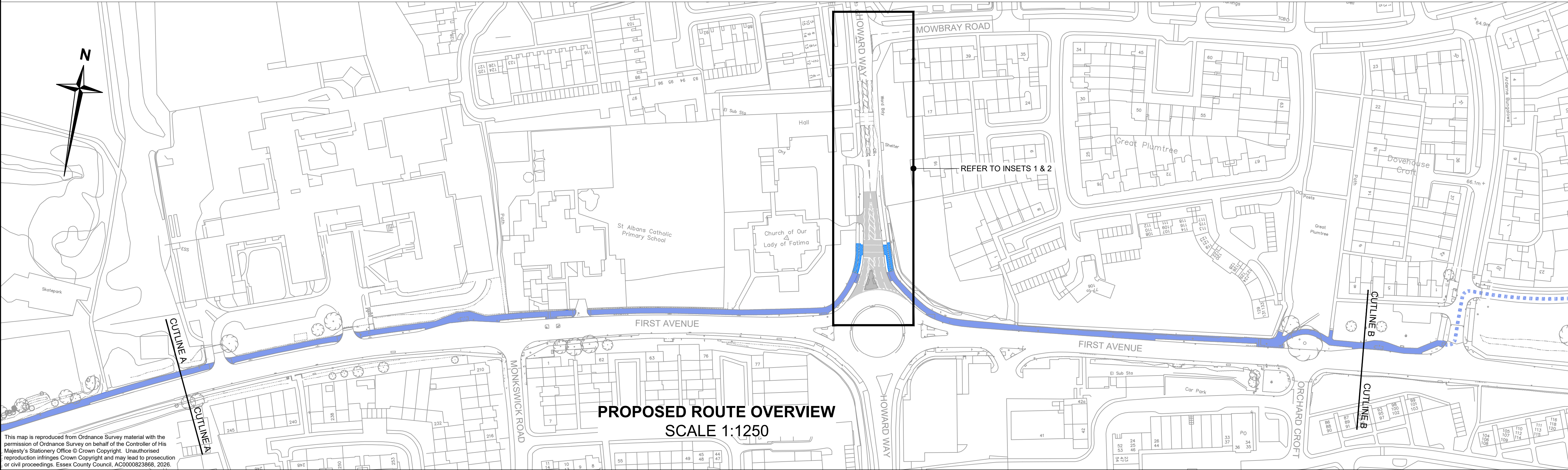
INSET 2 - PROPOSED LAYOUT SCALE 1:250
