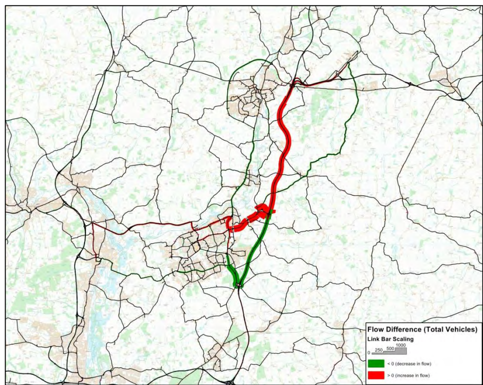
Medium Traffic Flow Difference between DM and DS 2021 models – IP (Overview)
