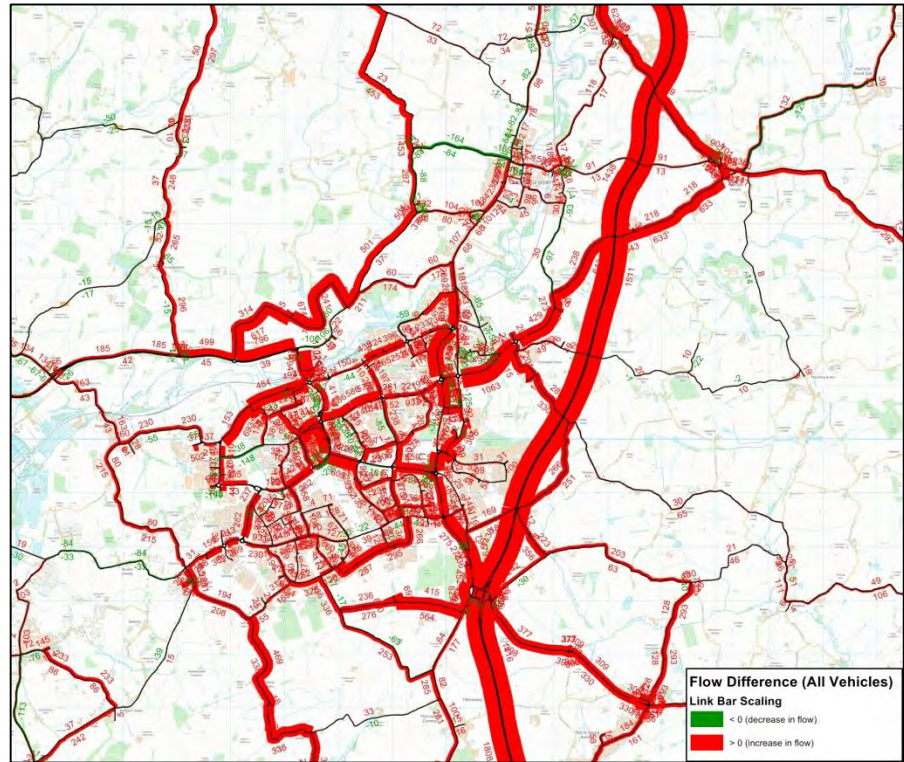
High Traffic Flow Difference between Base 2014 and DM 2036 models – AM (Harlow)
