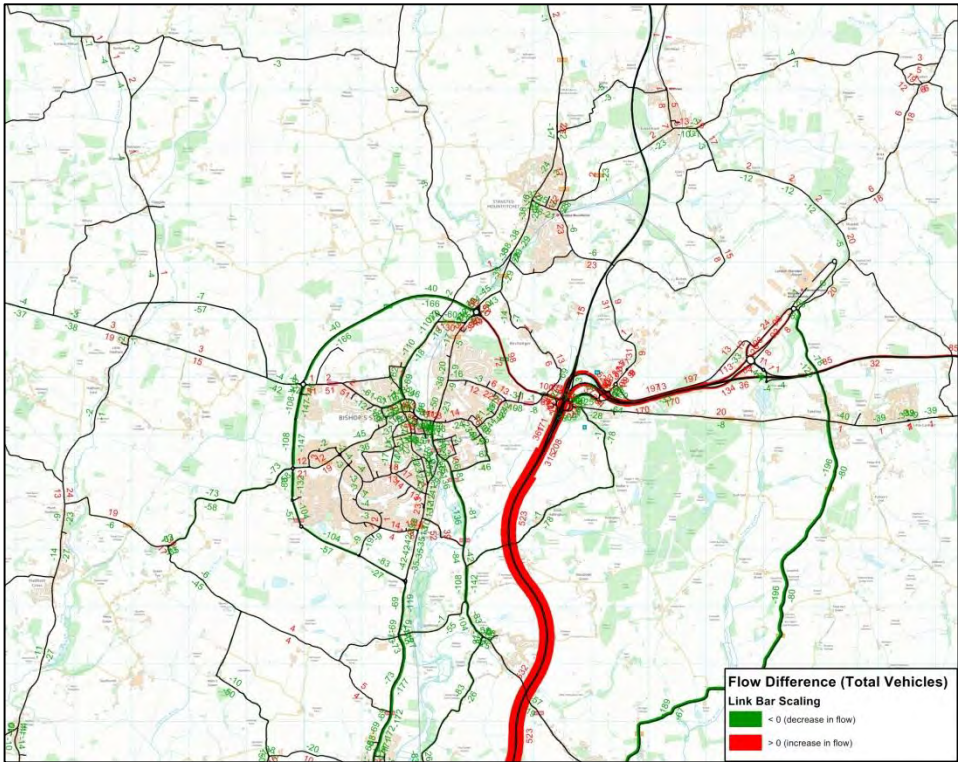
Medium Traffic Flow Difference between DM and DS 2021 models – PM (Bishop Stortford)
