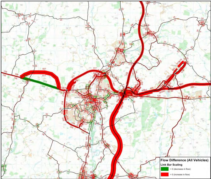
High Traffic Flow Difference between Base 2014 and DM 2021 models – PM (Bishop Stortford)
