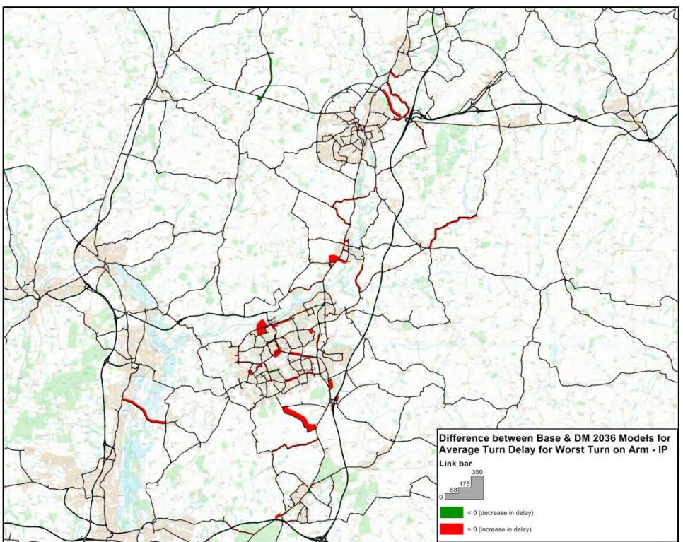
Medium Traffic Delay Difference between Base 2014 and DM 2036 models – IP (Overview)
