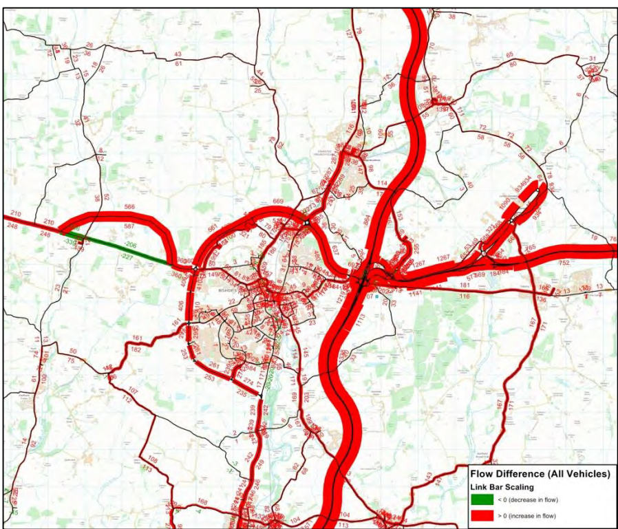
High Traffic Flow Difference between Base 2014 and DM 2036 models – IP (Bishop Stortford)
