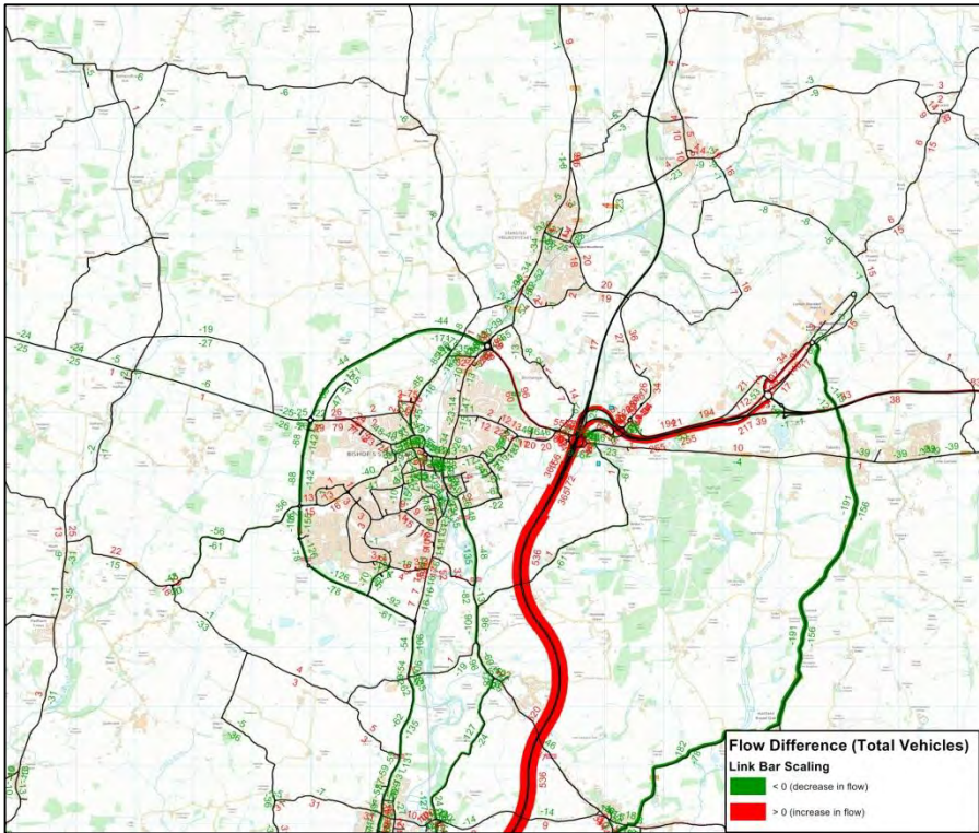
High Traffic Flow Difference between DM and DS 2021 models – PM (Bishop Stortford)
