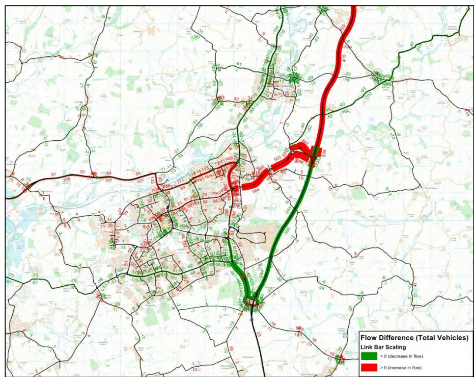
Medium Traffic Flow Difference between DM and DS 2021 models – IP (Harlow)
