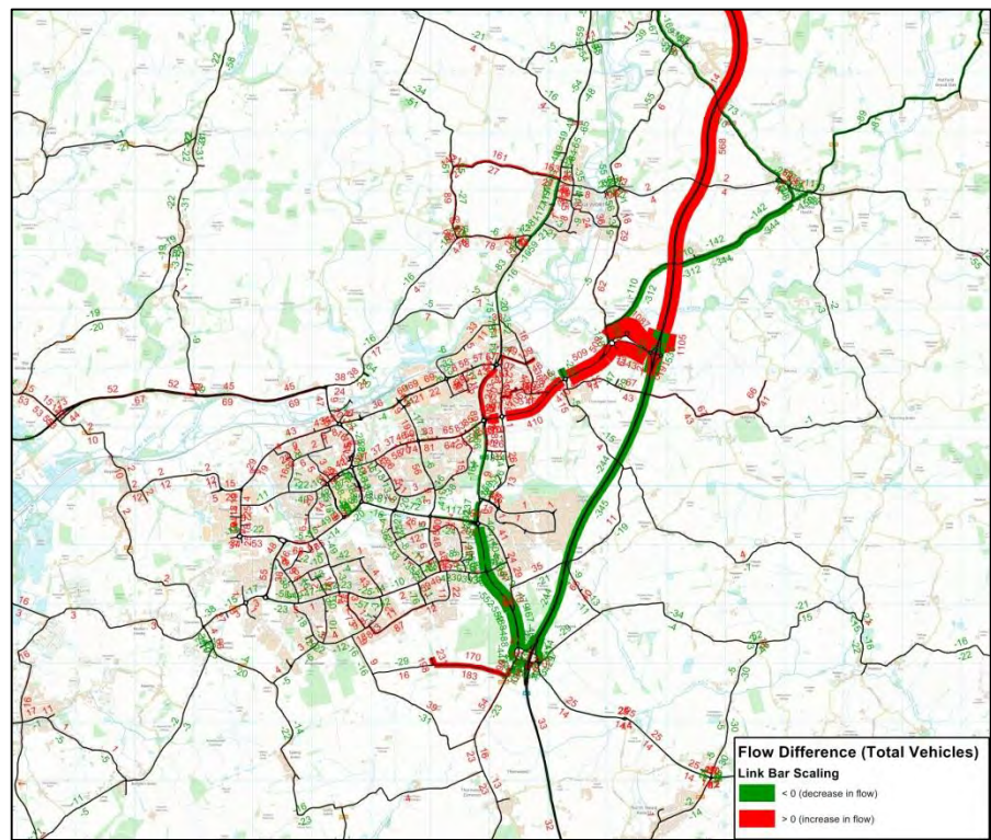
High Traffic Flow Difference between DM and DS 2021 models – AM (Harlow)
