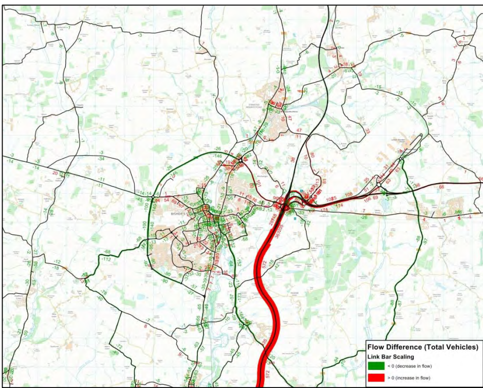
Medium Traffic Flow Difference between DM and DS 2021 models – AM (Bishop Stortford)
