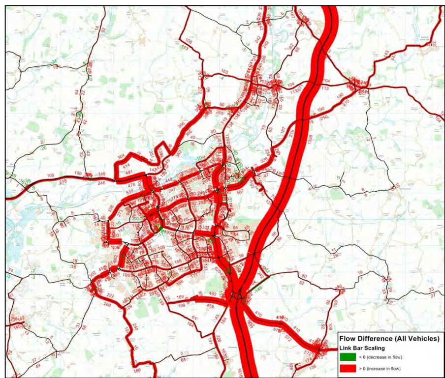
High Traffic Flow Difference between Base 2014 and DM 2036 models – IP (Harlow)
