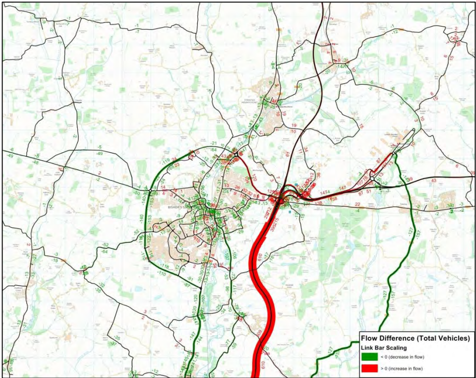
Medium Traffic Flow Difference between DM and DS 2036 models – IP (Bishop Stortford)
