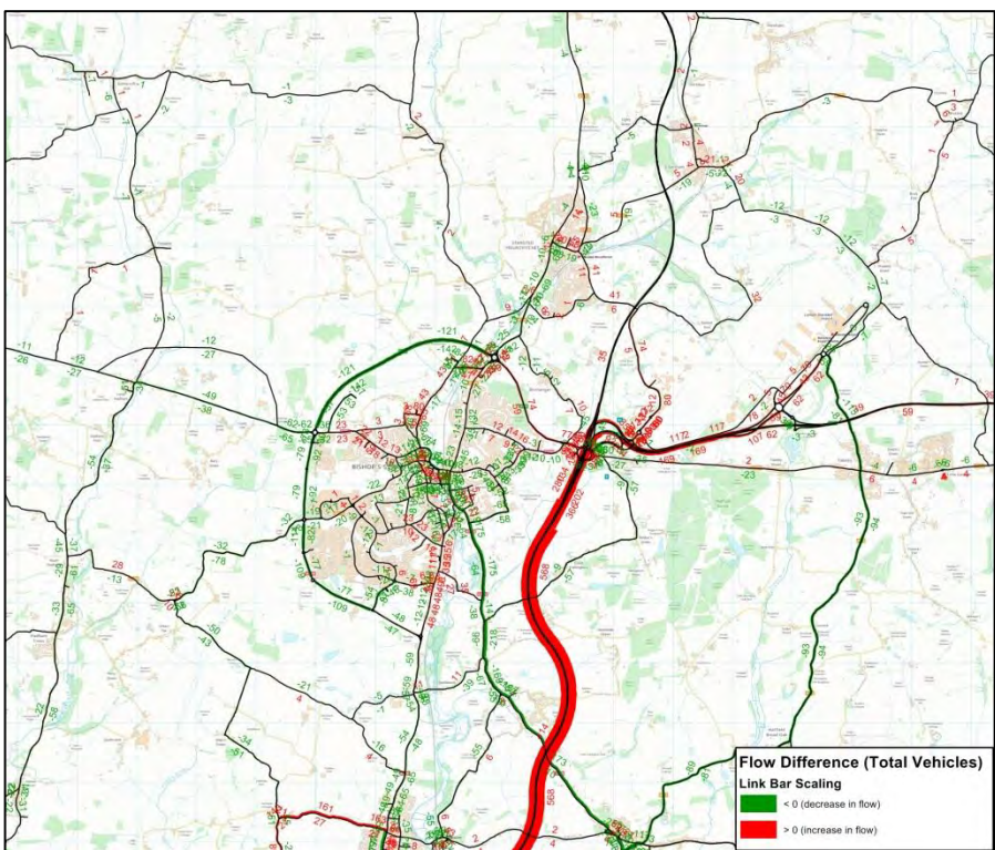
High Traffic Flow Difference between DM and DS 2021 models – AM (Bishop Stortford)
