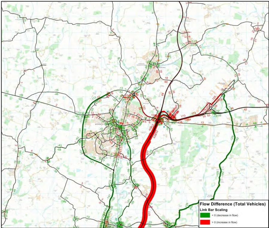
High Traffic Flow Difference between DM and DS 2036 models – IP (Bishop Stortford)
