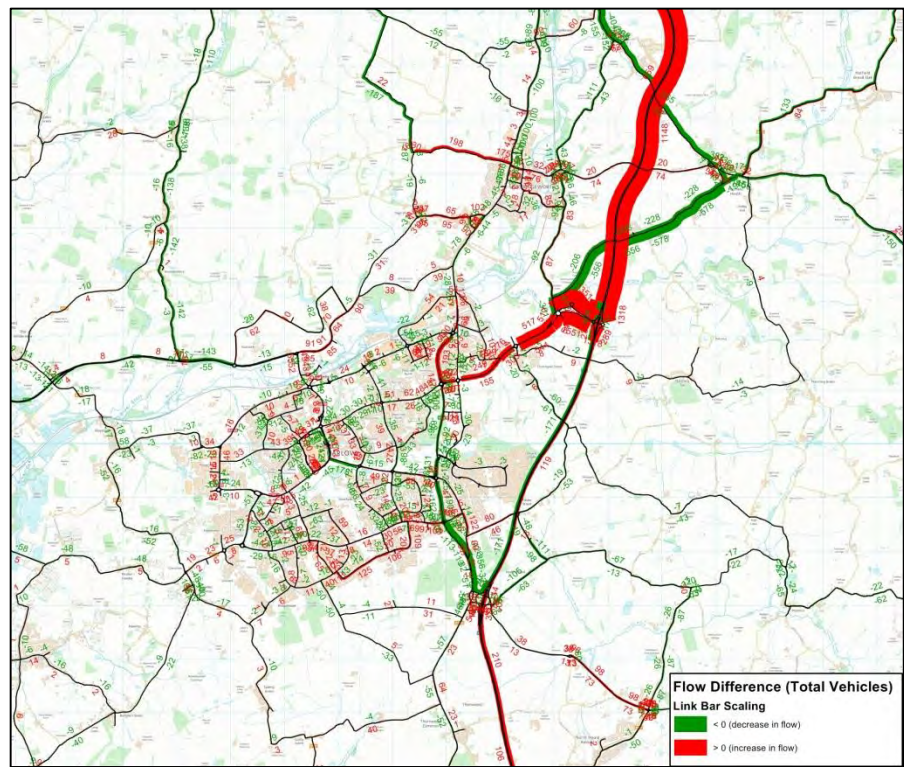
High Traffic Flow Difference between DM and DS 2036 models – AM (Harlow)
