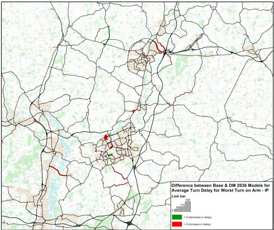
NTEM Traffic Delay Difference between Base 2014 and DM 2036 models – IP (Overview)
