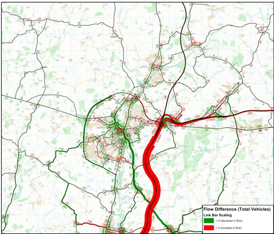
High Traffic Flow Difference between DM and DS 2036 models – AM (Bishop Stortford)
