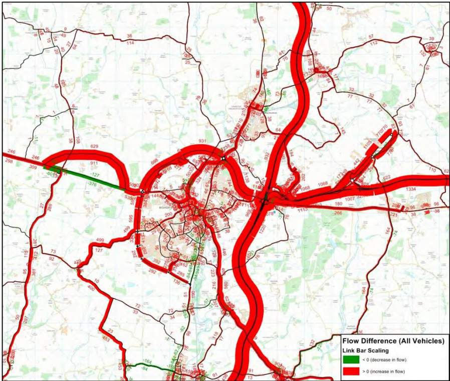
High Traffic Flow Difference between Base 2014 and DM 2036 models – AM (Bishop Stortford)
