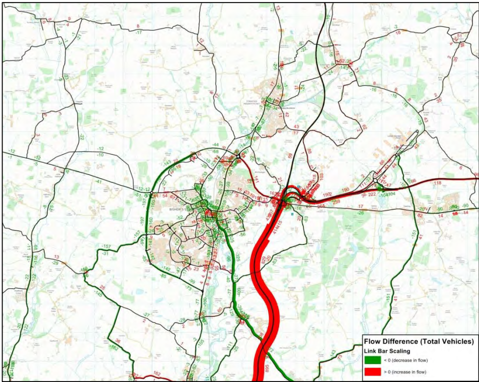
Medium Traffic Flow Difference between DM and DS 2036 models – AM (Bishop Stortford)
