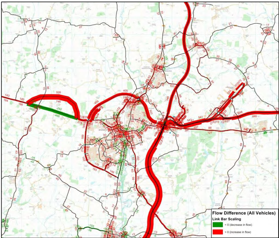
High Traffic Flow Difference between Base 2014 and DM 2021 models – AM (Bishop Stortford)
