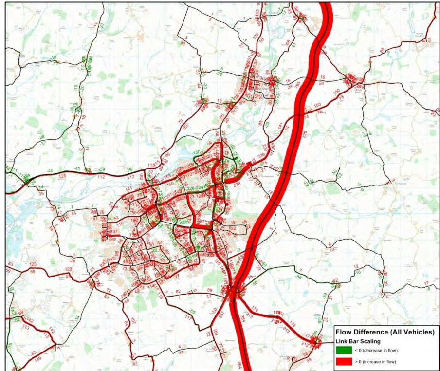
High Traffic Flow Difference between Base 2014 and DM 2021 models – PM (Harlow)
