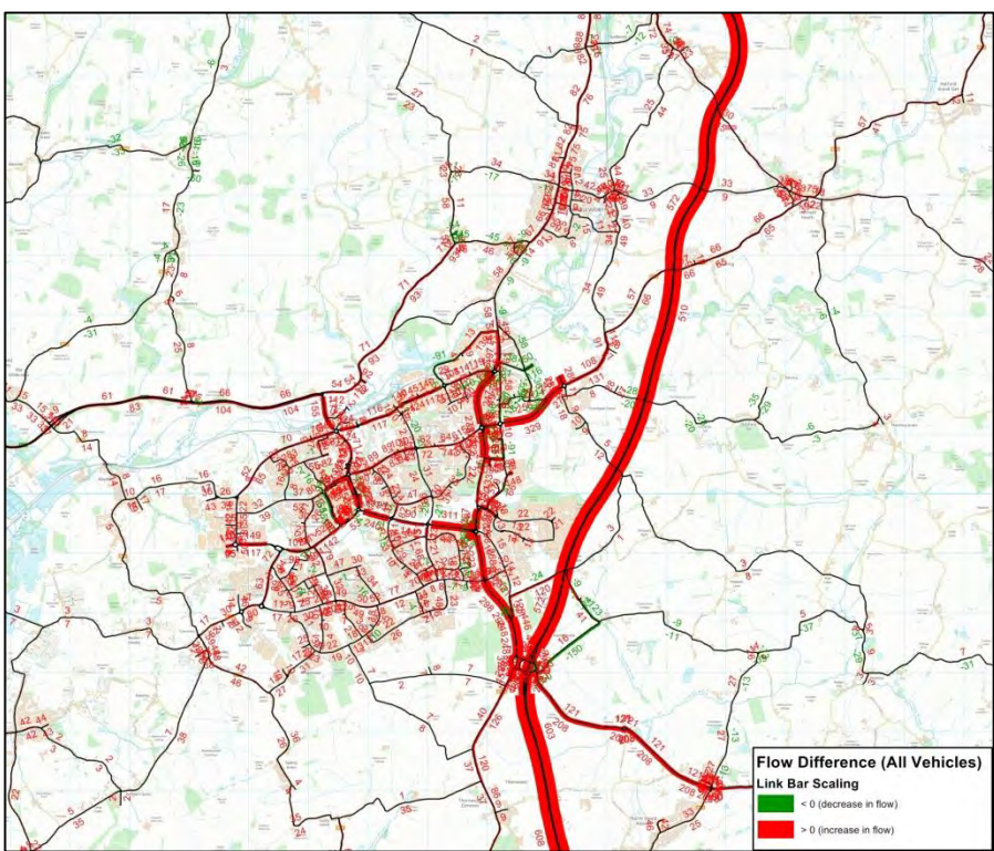
High Traffic Flow Difference between Base 2014 and DM 2021 models – IP (Harlow)
